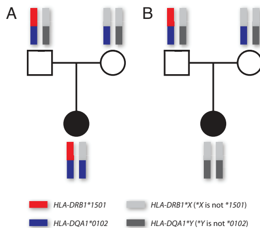
Fig. 1. Trans Epistasis between HLA-DRB1*1501 and HLA-DQA1*0102 . (A) HLA-DQA1*0102 (blue) is overtransmitted (OR = 2.1) when HLA-DRB1*1501 (red) is also present in affected offspring. (B) When HLA-DRB1*1501 is absent, HLA-DQA1*0102 is undertransmitted (OR = 0.64).
